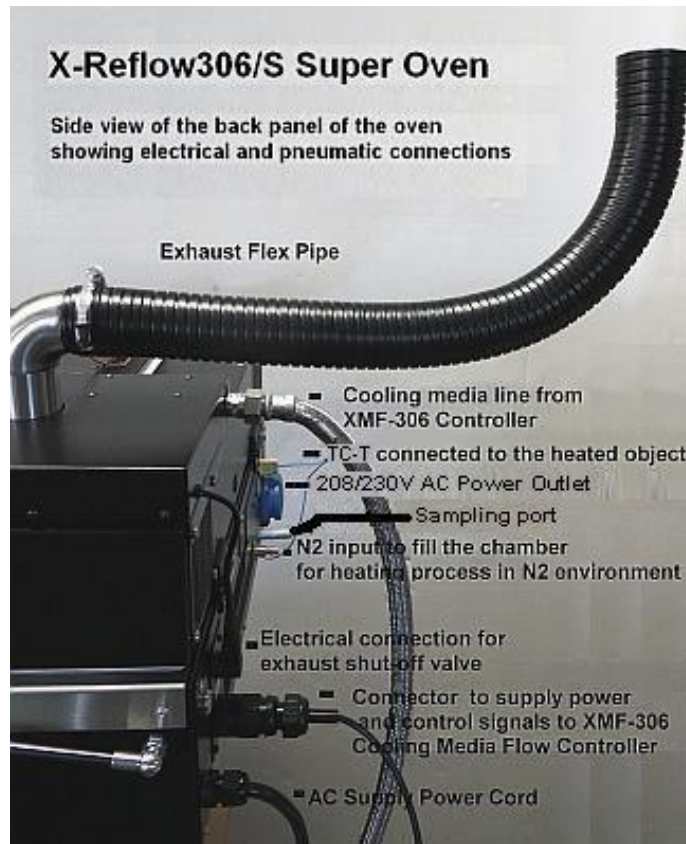
X-Reflow306/S rear panel side view
